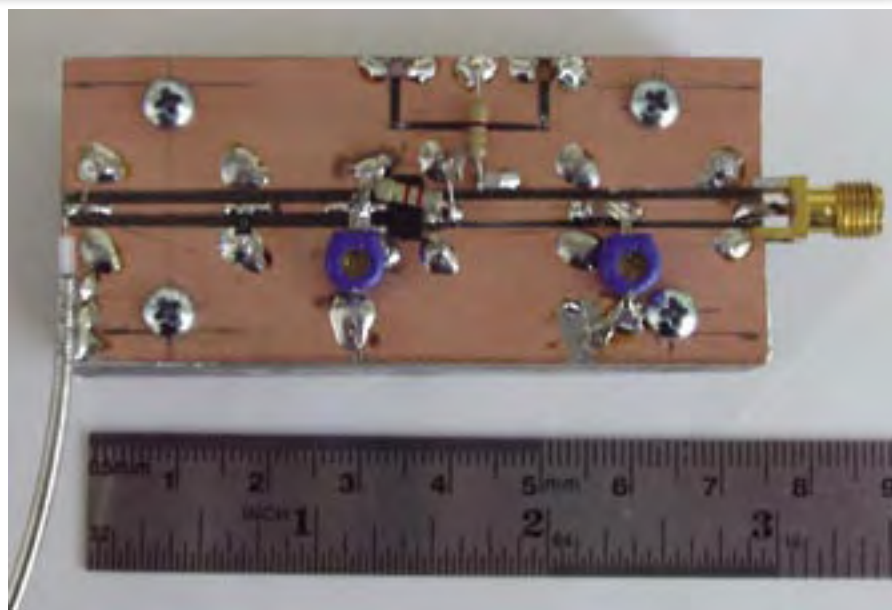
Component layout
