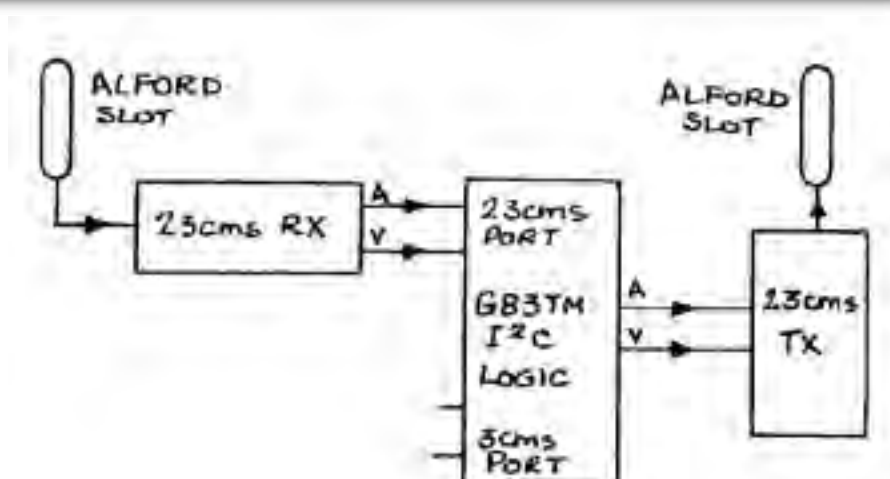
Figure 1 - 23cms ATV Repeater
